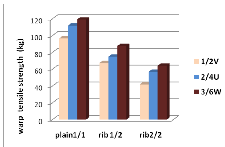
Figure (6) The effect of Pile Structure and Ground Weave on Warp Tensile Strength.
