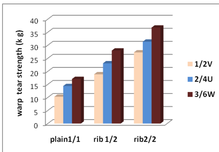
Figure (8): The Effect of Pile Structure and Ground Weave on Warp Tear Strength
