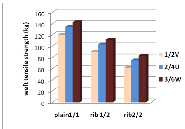
Figure (7): The Effect of Pile Structure and Ground Weave on Weft Tensile Strength
