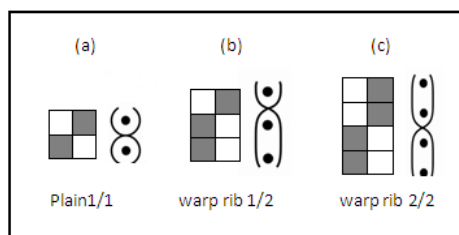
Figure (3) the famous weaves for the ground
