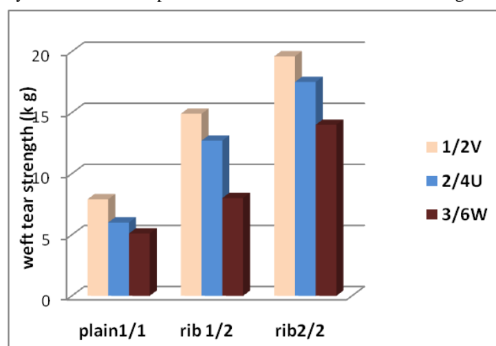
Figure (9) The effect of Pile Structure and Ground Weave on Weft Tear Strength.
