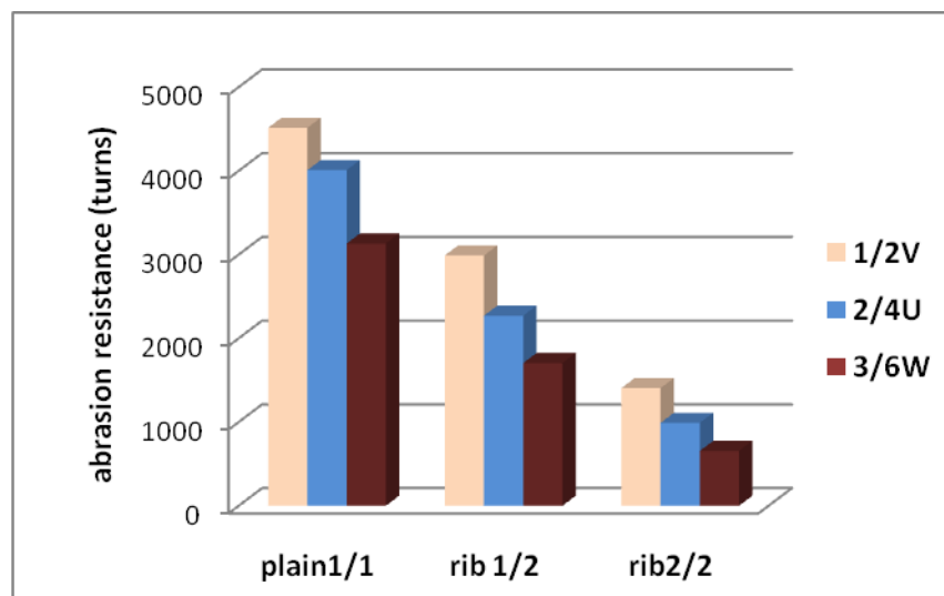
Figure (10): The Effect of Pile Structure and Ground Weave on Abrasion Resistance.
