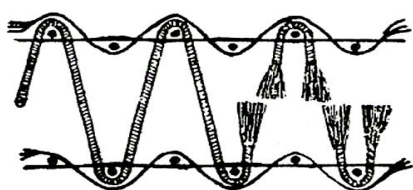
Figure (1) Face to face weaving principle
