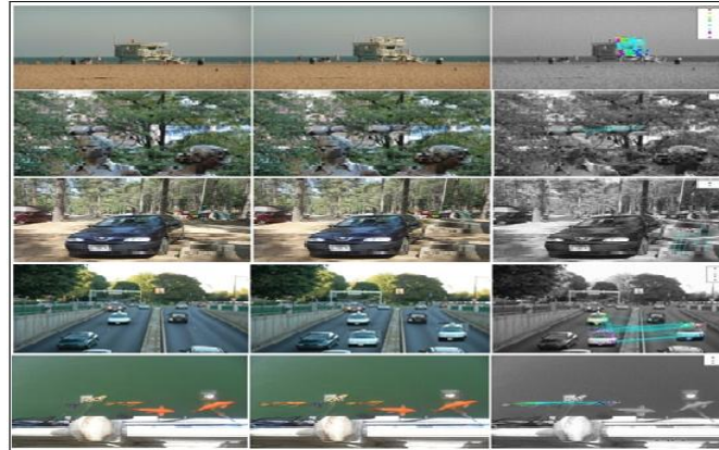
Figure 4:- Results of hybrid DCT plus SIFT on some forged images of additional dataset
