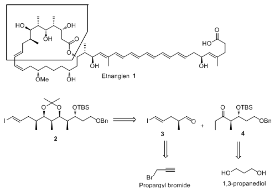
Fig 1: Retro Synthetic Analysis
