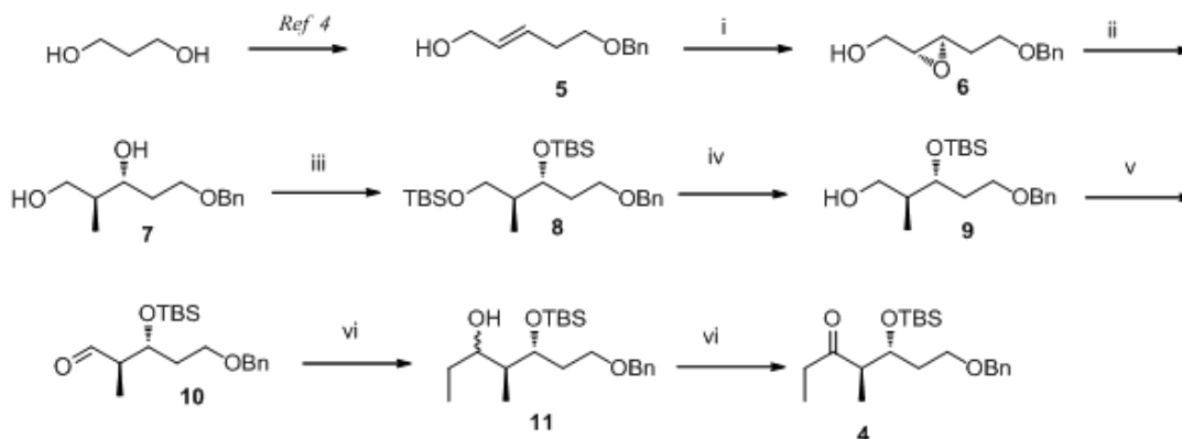
Fig 2: Synthesis of Fragment 4
