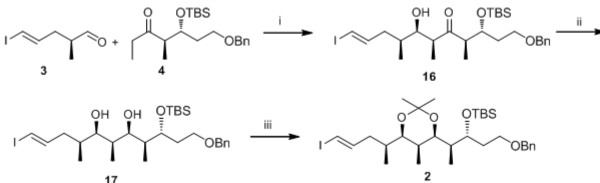
Fig 4: Coupling of aldehyde 3 ethyl ketone 4.
