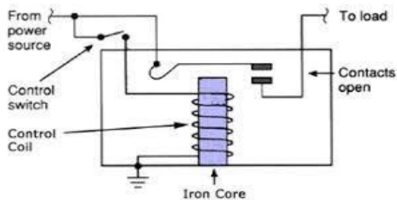
Fig -4: Power Relay
