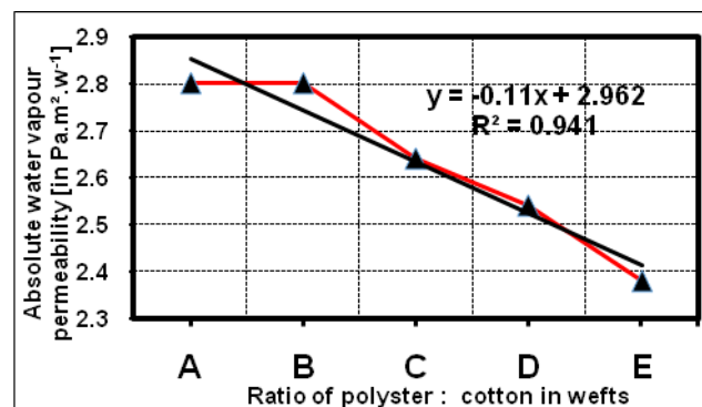
Fig. (9) Relation between polyester and cotton weft yarns blending ratio and Absolute water vapour permeability of fabric
