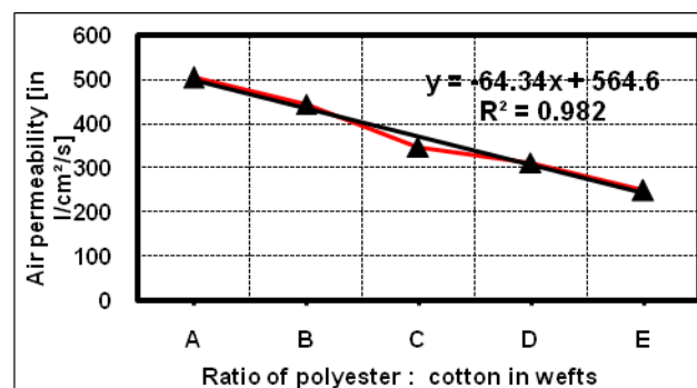
Fig. (7) Relation between polyester and cotton weft yarns blending ratio and fabric air permeability
