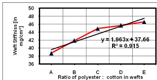
Fig. (6) Relation between polyester and cotton weft yarns blending ratio and weft stiffness
