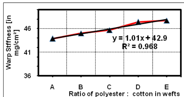
Fig. (5) Relation between polyester and cotton weft yarns blending ratio and warp stiffness
