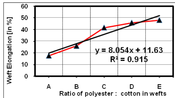
Fig. (4) Relation between polyester and cotton weft yarns blending ratio and weft elongation
