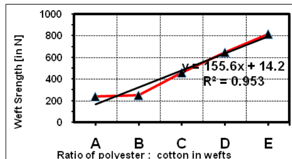
Fig. (2) Relation between polyester and cotton weft yarns blending ratio and weft tensile strength
