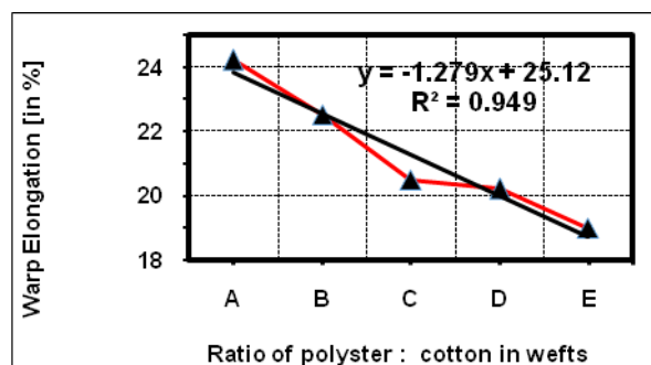
Fig. (3) Relation between polyester and cotton weft yarns blending ratio and warp elongation
