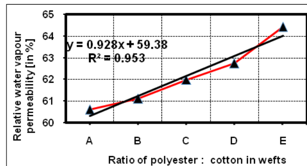
Fig. (8) Relation between polyester and cotton weft yarns blending ratio and Relative water vapour permeability of fabric
