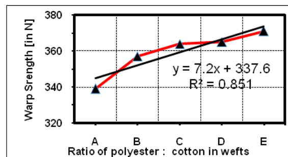
Fig. (1) Relation between polyester and cotton weft yarns blending ratio and warp tensile strength
