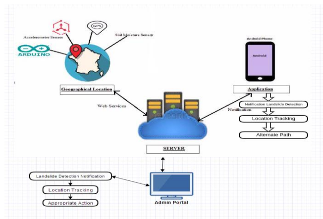
Figure 1 ARCHITECTURE DIAGRAM
