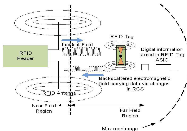
Fig. 3: RFID Communication
