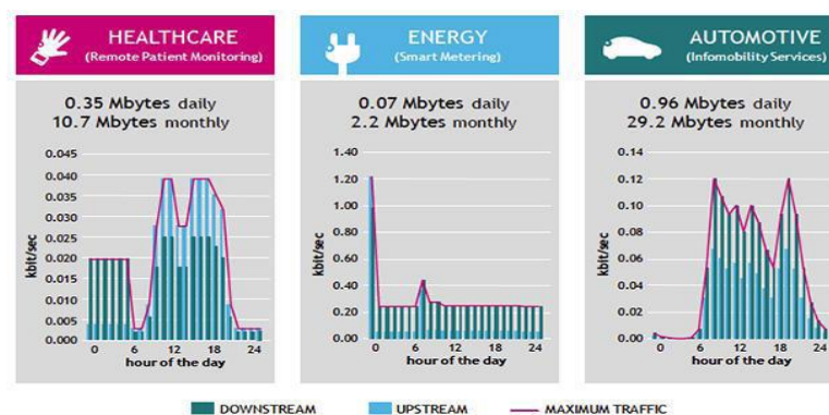
Fig. 6: Traffic Patterns for IoT Applications
