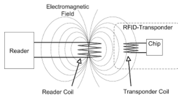
Fig. 2: RFID Basic Functioning
