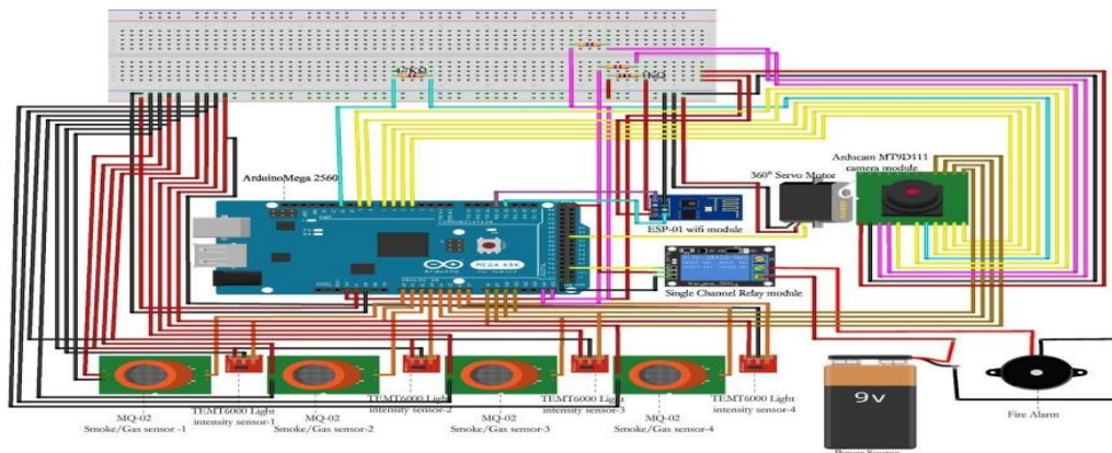
Fig.6.Circuit diagram of fire alarm system.
