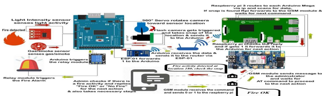
Fig.1. System Architecture.
