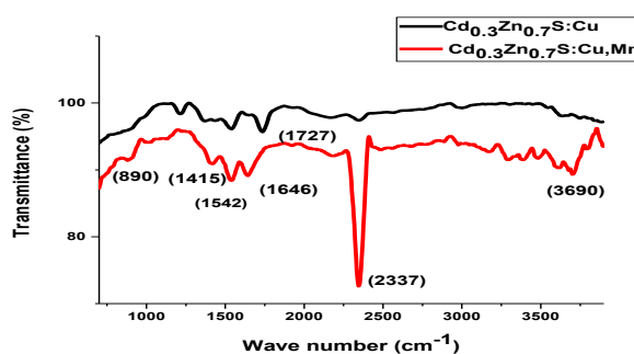
“Fig.2 FTIR spectra of Cu and Cu,Mn doped Cd 0.3 Zn 0.7 S nanomaterials.”
