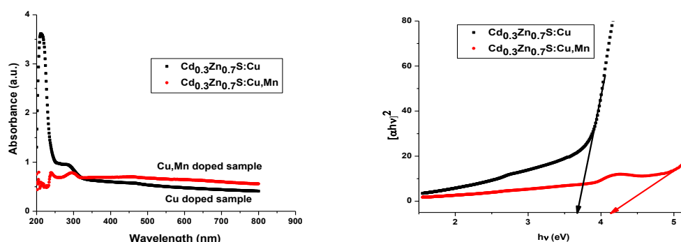
“Fig. 4 (a) UV-visible absorption spectra and (b) band gap energy of Cu and Cu,Mn doped \text{Cd}_{0.3}\text{Zn}_{0.7}\text{S} nanomaterials.”
