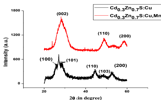
“Fig.1 XRD pattern of Cu and Cu,Mn doped \text{Cd}_{0.3}\text{Zn}_{0.7}\text{S} nanomaterials.”
